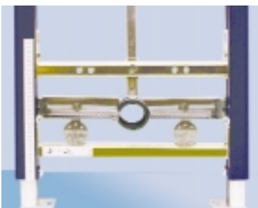
Fully adjustable bidet frame
